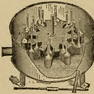
Fig. 60. BABCOCK'S MILK TESTING APPARATUS.
